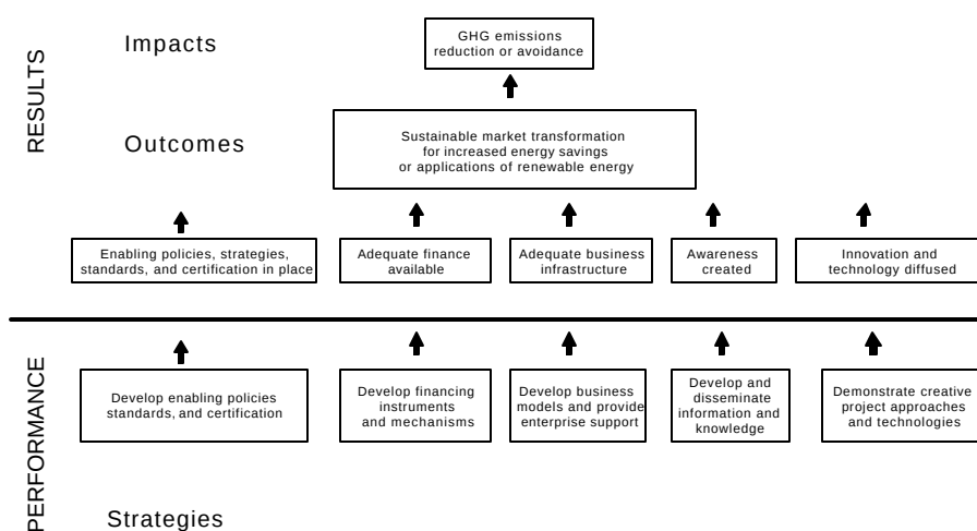
Figure 1.1: Evaluation framework
