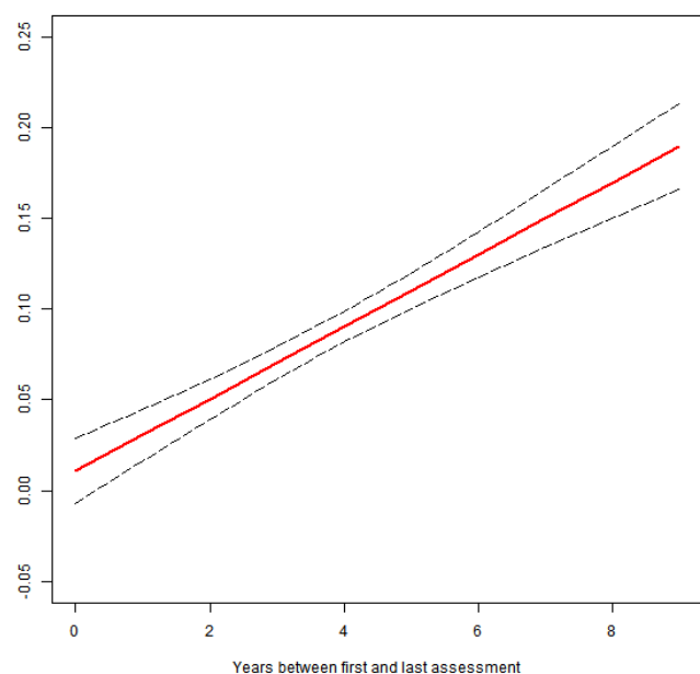
Figure 9 Estimated correlation between the number of years between assessments and changes in scores
