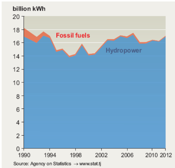
Figure 2. Power generation
