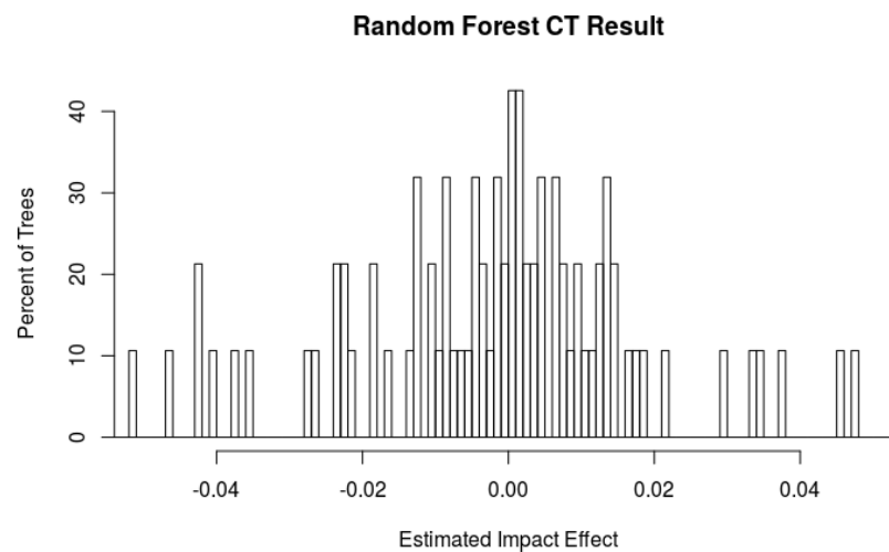
Figure 14: The result of a random forest for one GEF observation. Each of 1000 iterations are plotted
