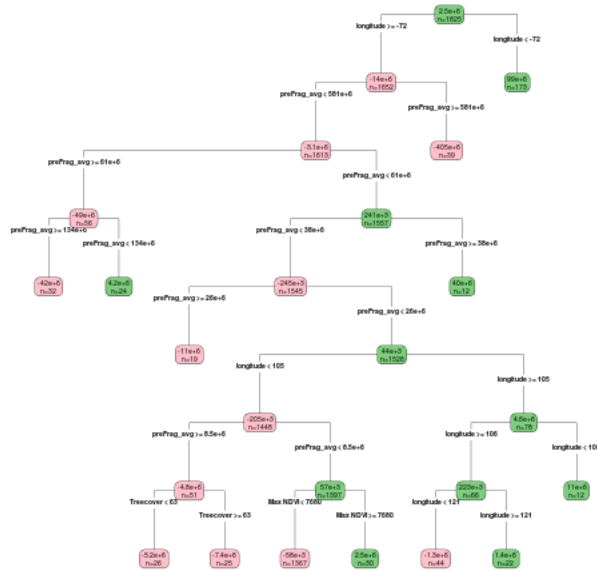
Figure 8: A Causal Tree representing impacts of GEF LD Projects on forest fragmentation (for easier viewing, an online application is available at http://labs.aiddata.org/GEF/treeBrowser/ ).
