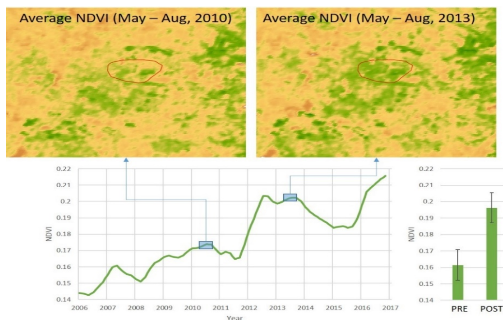
Figure 11: NDVI Change at Haba Lake Reserve, China (GEF ID 2369)
