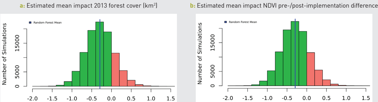
FIGURE 2: Model uncertainty
