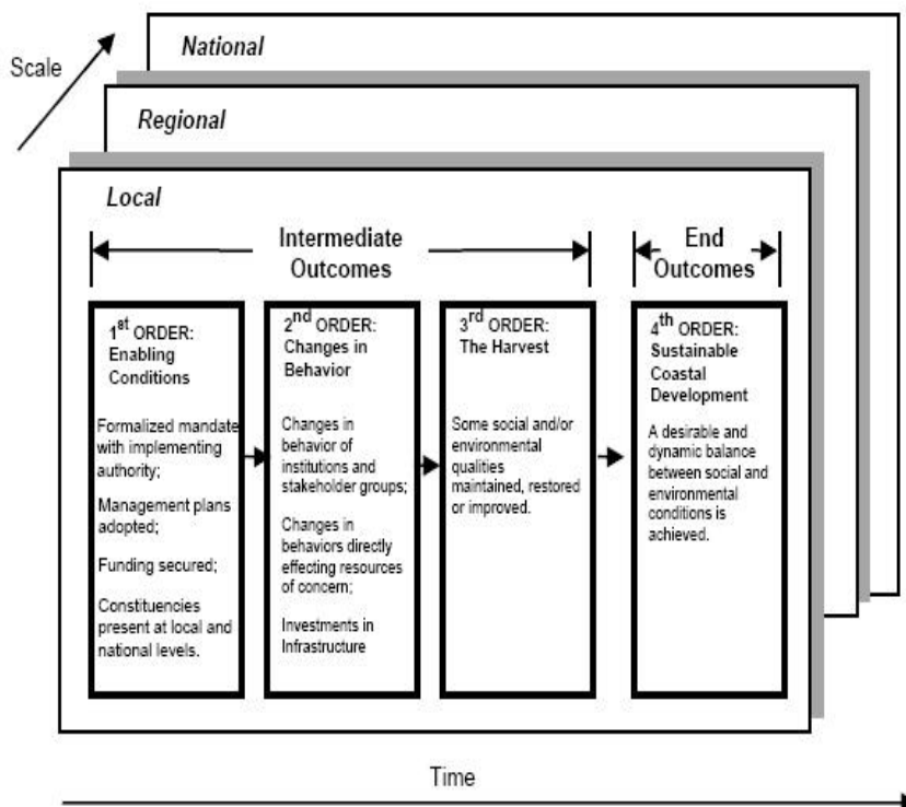
Fig. 1. The four orders of coastal governance outcomes. Adapted from [2].
